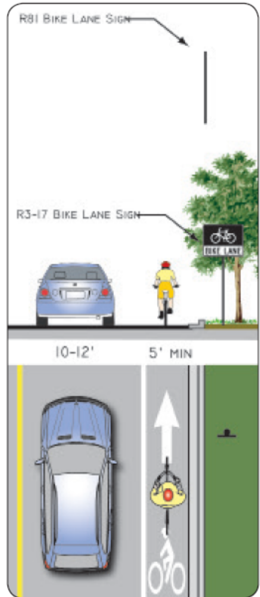
Recommend bike lane without on-street parking design.
