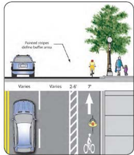
Recommended buffered bike lane design.
