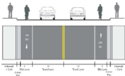
32' Road Curb-to-Curb Width
