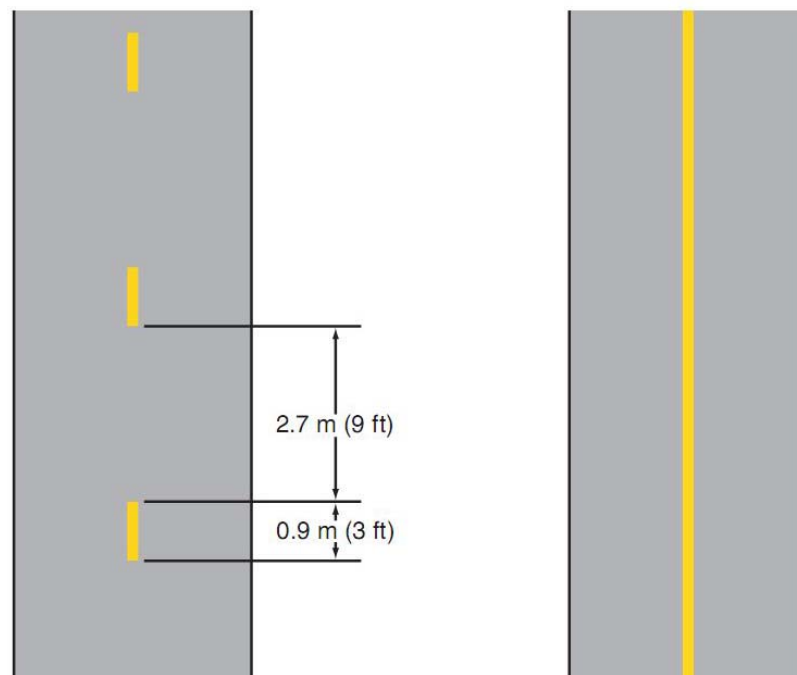
Figure 1719: Examples of Centerline Markings for Trails
