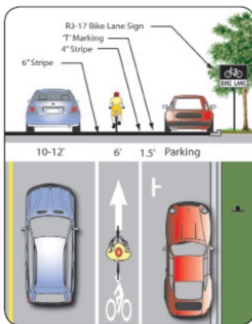
Parking buffer bike lane design.
