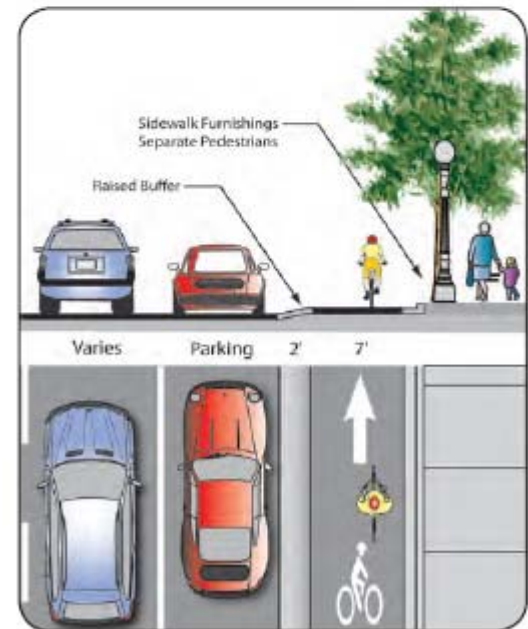
Recommended cycle track design with on-street parking.
