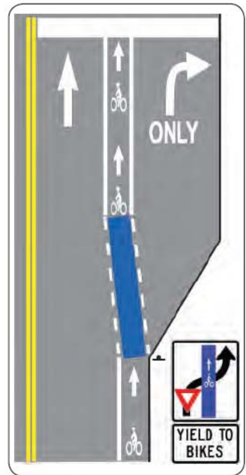
Recommended colored bike lane design.
