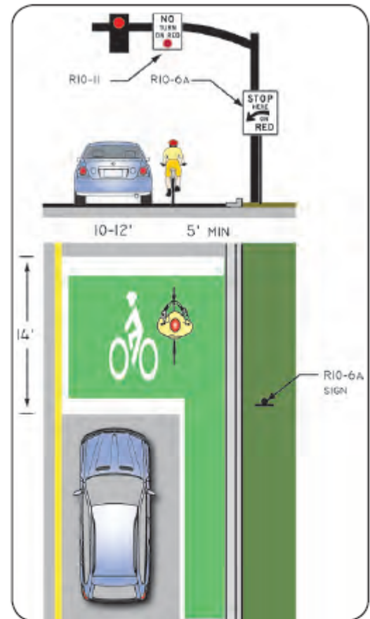
Recommended bike box design.
