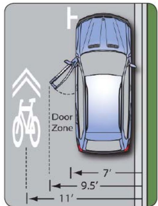
Shared lane marking placement guidance for streets with on-street parking.
