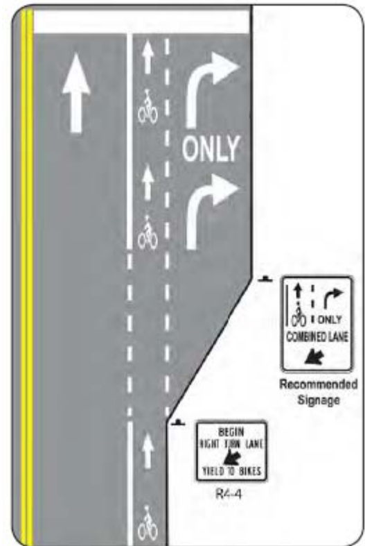
Recommended shared bike/right turn lane design.
