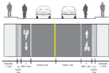
32' Road Curb-to-Curb Width
