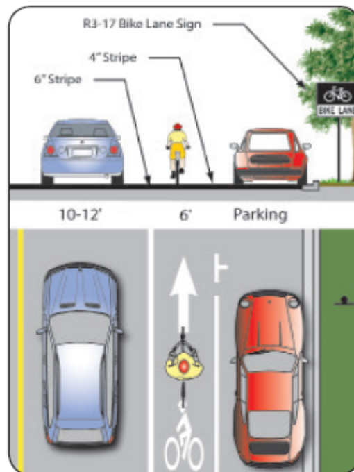
Parking 'T' bike lane design.
