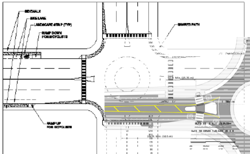
Recommended bike lane at roundabout design.
