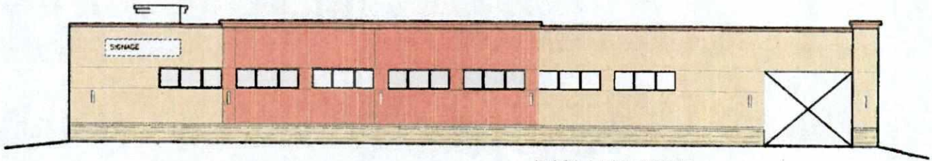
EAST ELEVATION
