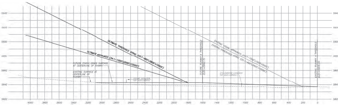
RUNWAY 4 - PROFILE
