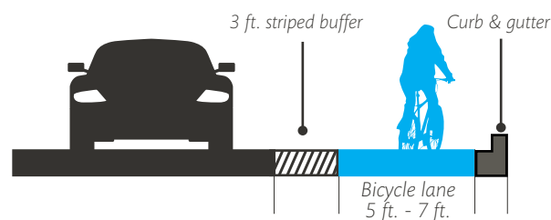
FIGURE 7.4.75 Bicycle Lane
