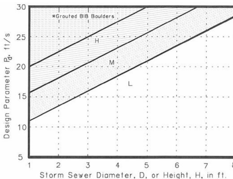
FIGURE 6.10.27 Low Tailwater Rip-rap Basins for Storm Sewer Pipe Outlets - Rip-rap Selection Chart for Low Tailwater Basin at Pipe Outlet
