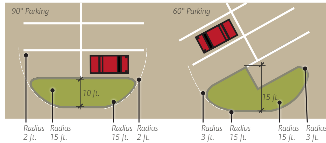
FIGURE 7.4.122 Parking Islands
