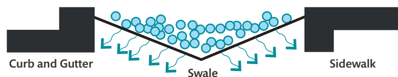
FIGURE 6.12.39 Swale Diagram
