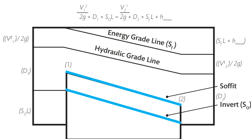
FIGURE 6.10.13 Hydraulic Grade
