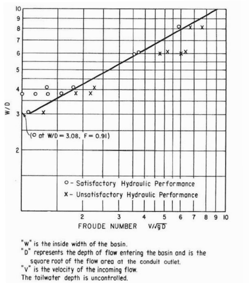
FIGURE 6.10.17 Basin Width Diagram for U.S.D.I. Bureau of Reclamation Type VI Impact Sill Basin
