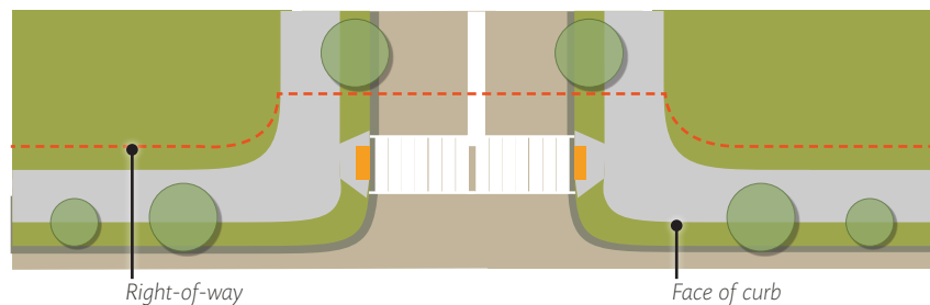
FIGURE 7.4.54 Right-of-way Dedication
