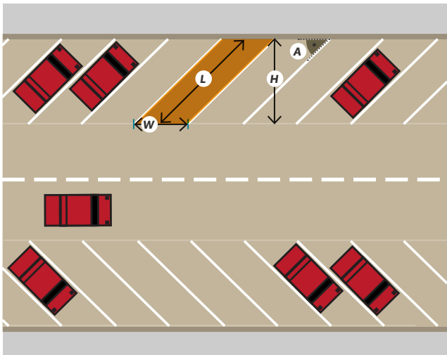
FIGURE 7.4.118 Dimensions for Angle Parking
