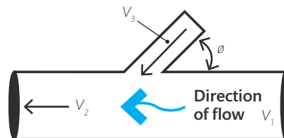
FIGURE 6.10.15 Junction Losses
