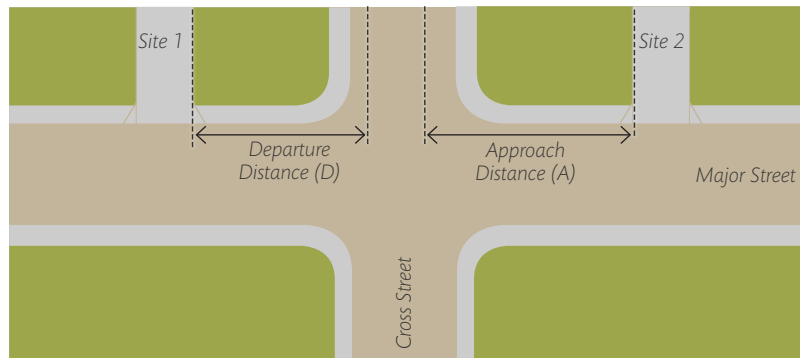
FIGURE 7.4.58 Commercial Site Access Points and Distance From Intersection
