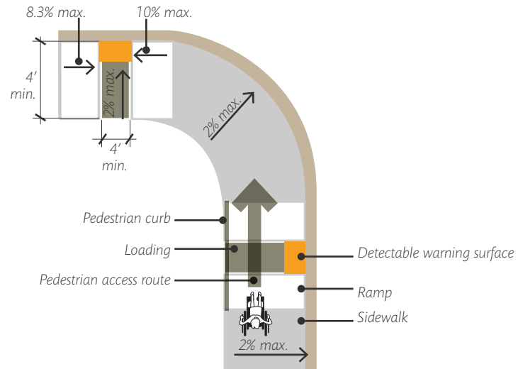
FIGURE 7.4.68 Parallel Curb Ramp
