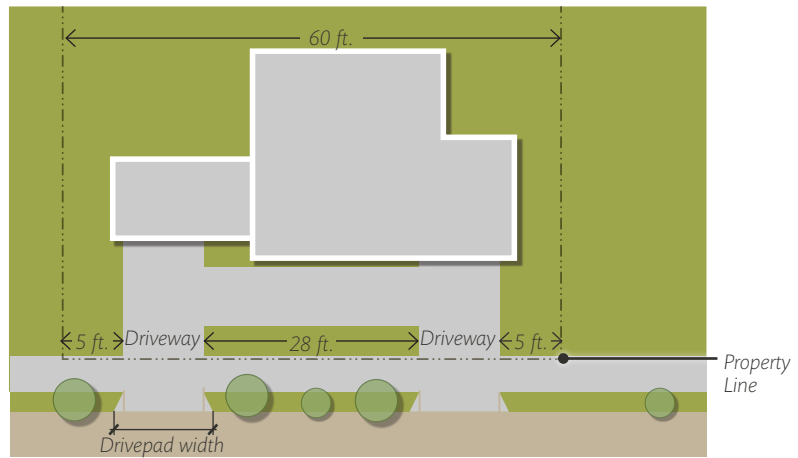
FIGURE 7.4.55 Low-density Residential Driveway Location and Dimensions
