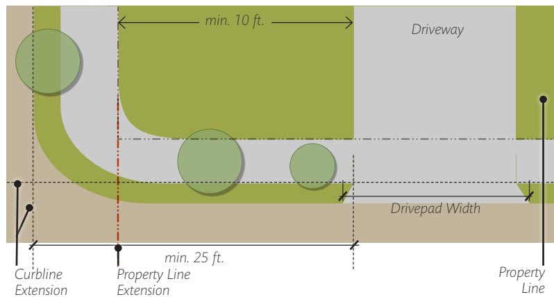
FIGURE 7.4.56 Driveway Distance From Intersection
