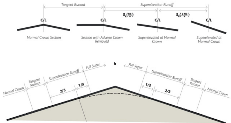
FIGURE 7.4.91 Example Superelevation Runout Plan
