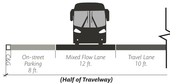
FIGURE 7.4.83 Travel Lane
