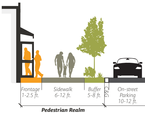
FIGURE 7.4.64 Mixed-use Area
