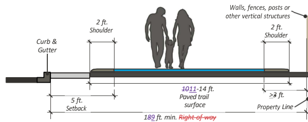
FIGURE 7.4.76 Paved Trail
