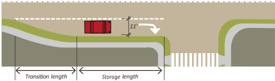
FIGURE 7.4.100 Right-turn Lane Design Elements
