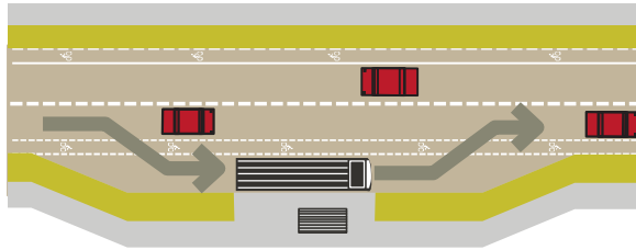
FIGURE 7.4.85 Bus Bay
