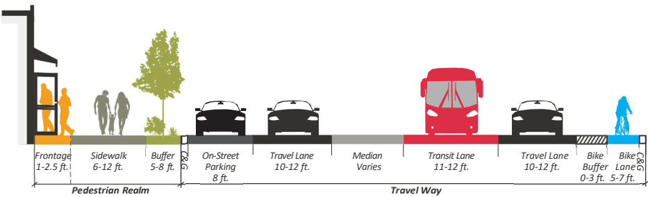
FIGURE 7.2.41 Street Element Dimensions Along Major Roads
