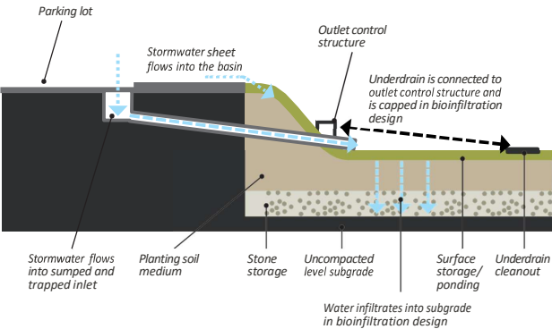
FIGURE 6.12.32 Depressed Bioretention Areas
