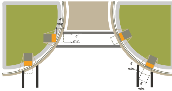
FIGURE 7.4.71 Curb Ramp Clear Space
