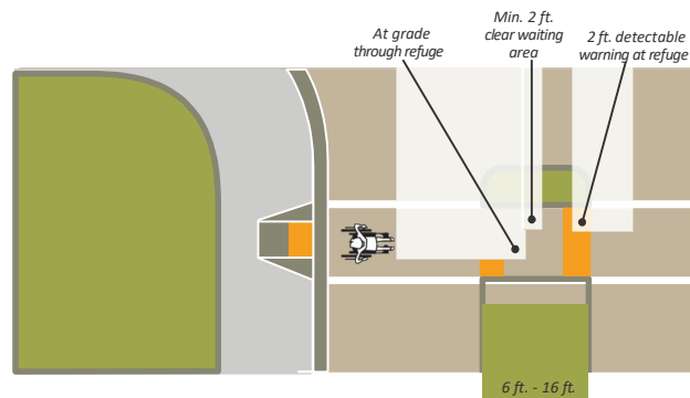
FIGURE 7.4.73 Refuge Island – At Grade
