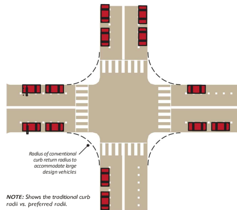
FIGURE 7.4.95 Standard Curb Return Radii Diagram
