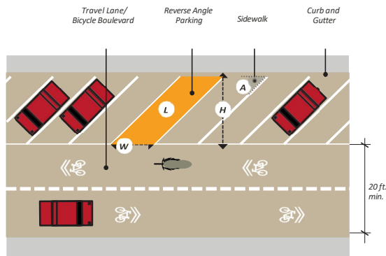
FIGURE 7.4.87 Dimensions for Angle Parking
