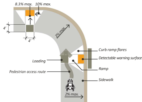
FIGURE 7.4.67 Perpendicular Curb Ramp
