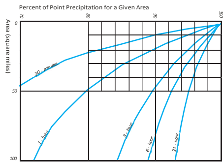
FIGURE 6.2.6 Depth - Area Curves
