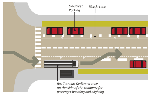
FIGURE 7.4.84 Bus Turnout
