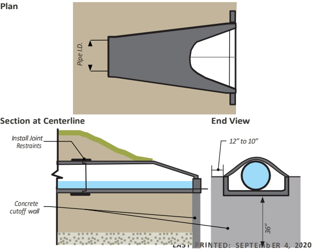
FIGURE 6.10.24 Concrete Flared End Section with Cutoff Wall for All Pipe Outlets
