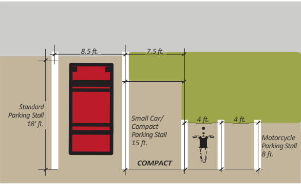
FIGURE 7.4.116 Parking Stall Dimensions
