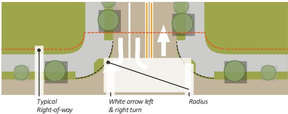
FIGURE 7.4.59 Curb Return Access Point
