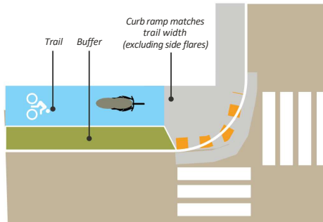
FIGURE 7.4.77 Blended Transition Ramp with Matching Trail and Ramp Width
