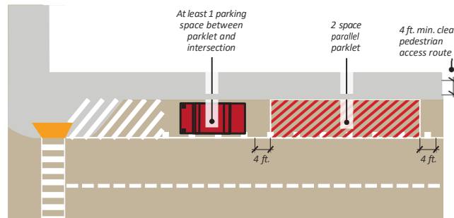
FIGURE 7.4.90 Parklet Location and Examples
