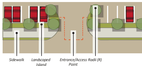
FIGURE 7.4.119 Site Access Design
