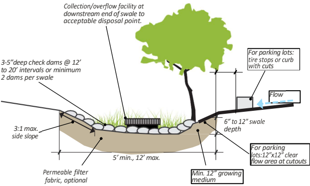
FIGURE 6.12.30 Depressed Parking Island
