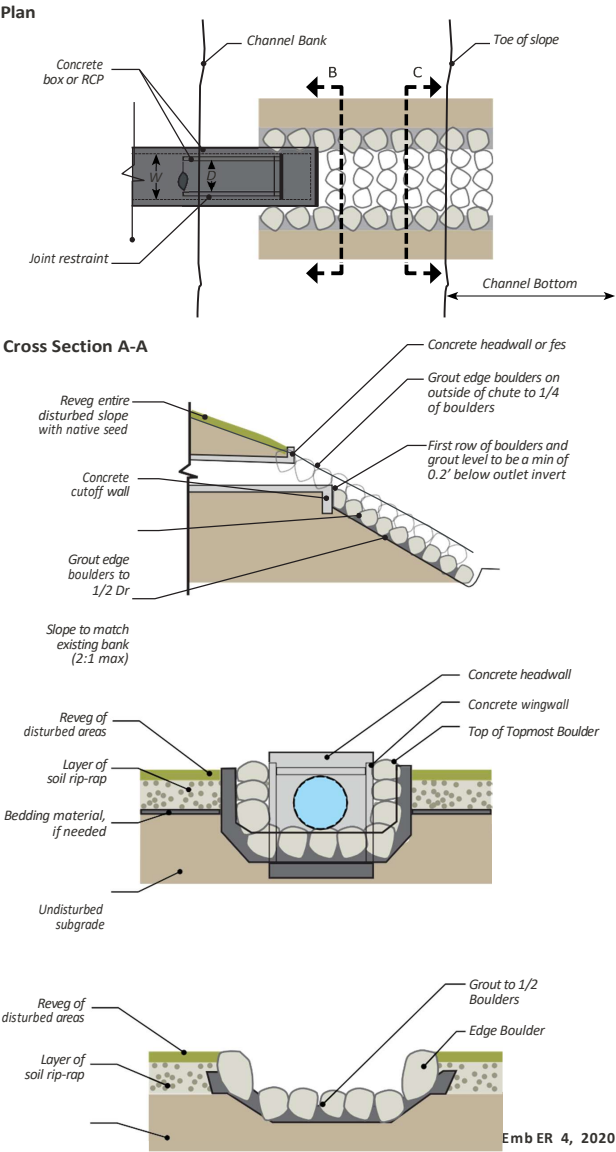
FIGURE 6.10.21 Grouted Boulder Rundown
