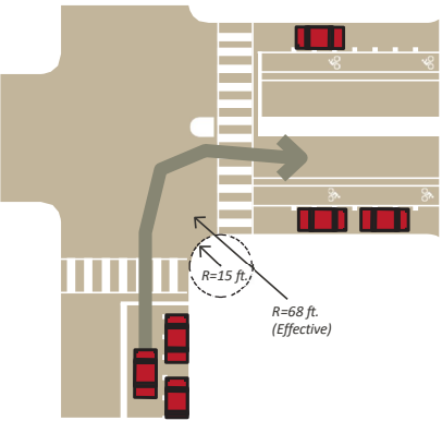
FIGURE 7.4.96 Effective Curb Return Radii Diagram
