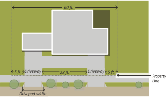
FIGURE 7.4.55 Low-density Residential Driveway Location and Dimensions
