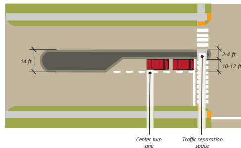
FIGURE 7.4.97 Median with Center Turn Lane
