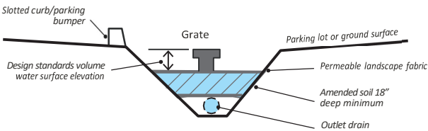
FIGURE 6.12.31 Depressed Parking Island Diagram
