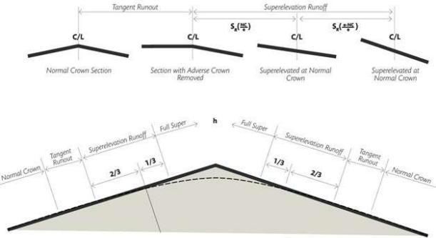
FIGURE 7.4.91 Example Superelevation Runout Plan
