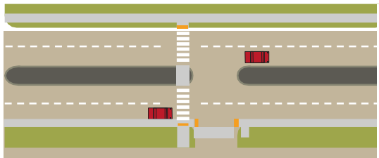
FIGURE 7.4.48 Uncontrolled Pedestrian Crossing Example
