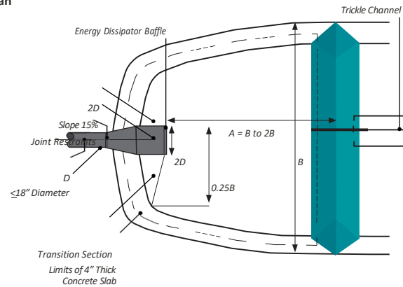
FIGURE 6.10.19 Impact Stilling Basin for Pipes Smaller than 18 Inches in Diameter Upstream of Forebays
