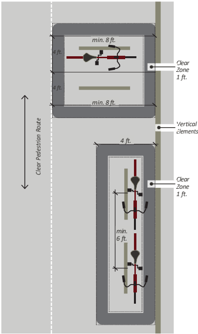
FIGURE 7.4.115 Bicycle Parking Stall Layout Options
