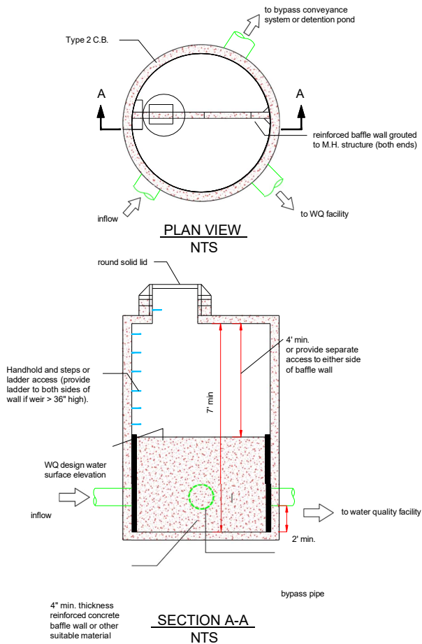
FIGURE 6.12.40 Splitter Manhole
