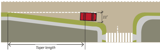
FIGURE 7.4.101 Right Taper Design Elements
