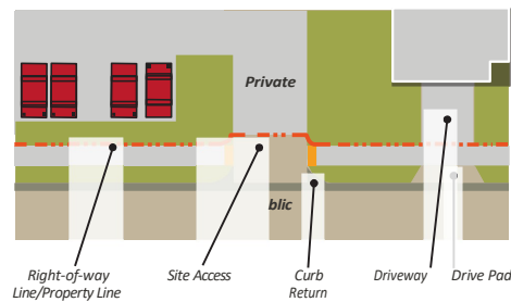
FIGURE 7.4.53 Site Access Elements
