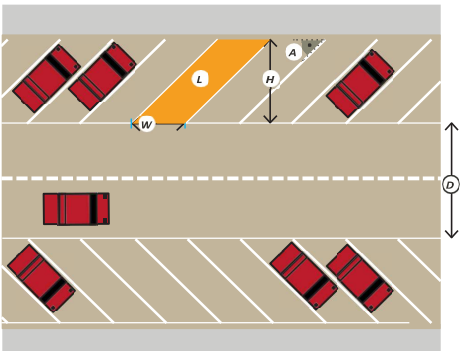
FIGURE 7.4.118 Dimensions for Angle Parking
