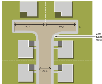
FIGURE 7.4.114 Hammerhead Dimensions
