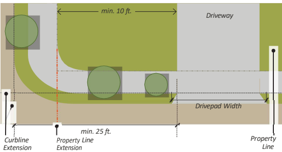
FIGURE 7.4.56 Driveway Distance From Intersection
