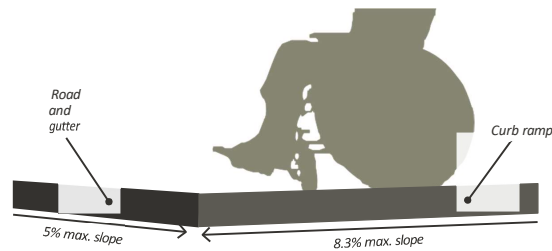
FIGURE 7.4.70 Curb Ramp Counter Slope
