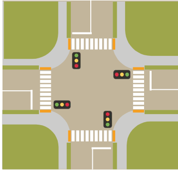
FIGURE 7.4.47 Controlled Pedestrian Crossing Example
