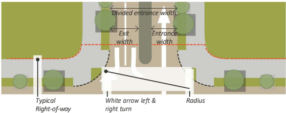
FIGURE 7.4.60 Divided Entrance Width
