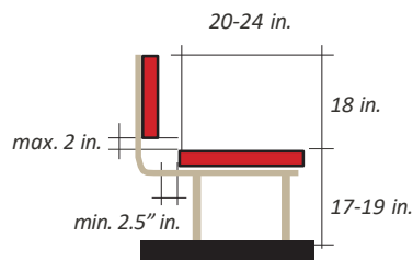
FIGURE 7.4.82 ADA/PROWAG-compliant Bench Design Requirements
