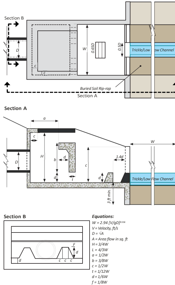
FIGURE 6.10.16 General Design Dimensions for U.S.D.I. Bureau of Reclamation Type VI Impact Sill Basin
