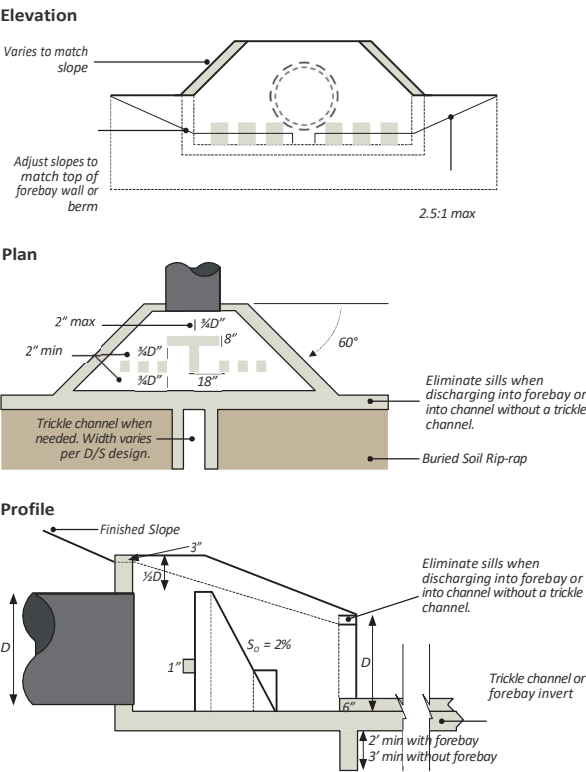
FIGURE 6.10.18 Modified Impact Sill Basin for Conduits 18-48 Inches in Diameter
