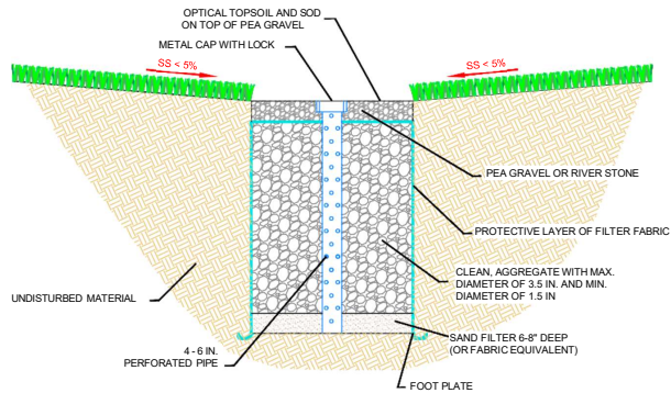
FIGURE 6.12.34 Infiltration Trench with Aggregate
