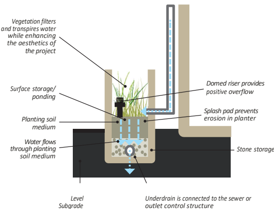
FIGURE 6.12.38 Planter Boxes Diagram
