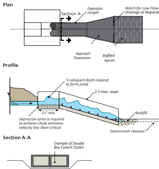
FIGURE 6.10.20 Baffle Chute Pipe Outlet
