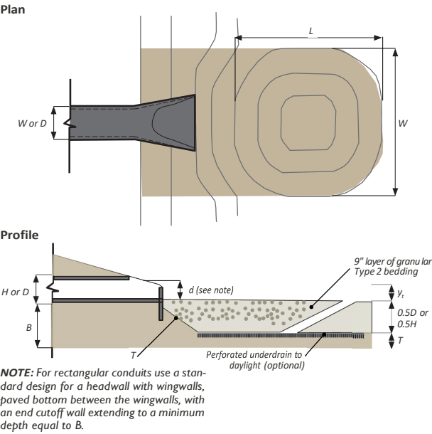
FIGURE 6.10.23 Low Trailwater Rip-rap Basins for Storm Sewer Pipe Outlets (HS-19)
