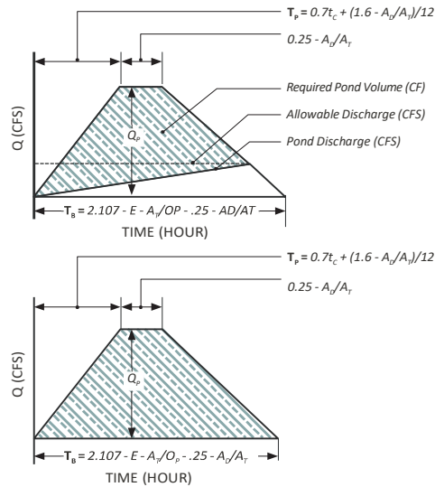
FIGURE 6.2.5 Time to Peak in 10-years
