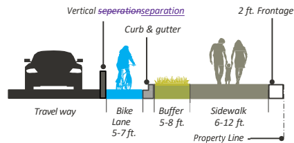
FIGURE 7.4.78 Trail Alternative 1, Vertical Separation
