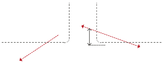
FIGURE 7.4.93 Intersection Sight Distance
