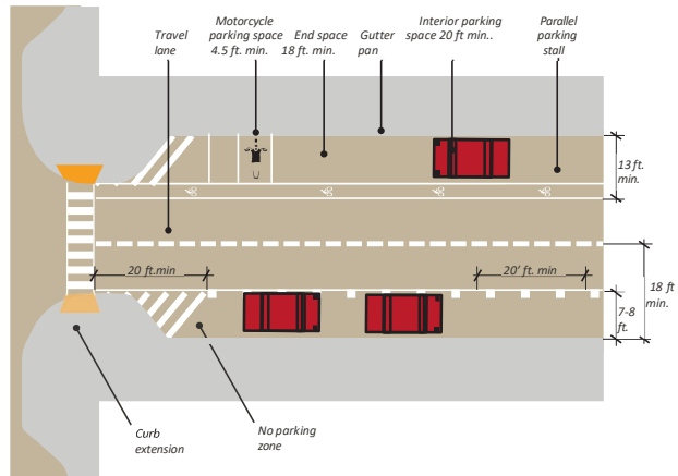
FIGURE 7.4.88 Parallel Parking Dimensions
