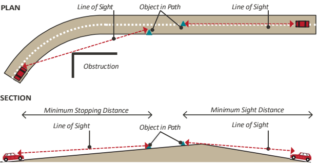
FIGURE 7.4.92 Stopping Sight Distance
