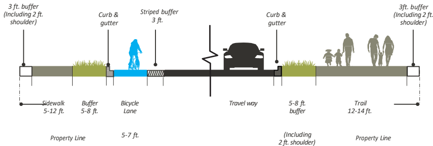
FIGURE 7.4.79 Trail Alternative 2, Trail in Lieu of Sidewalk
