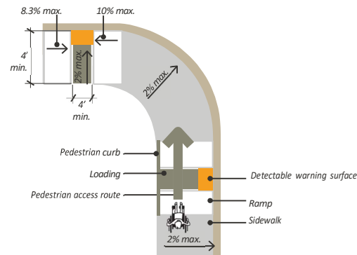
FIGURE 7.4.68 Parallel Curb Ramp
