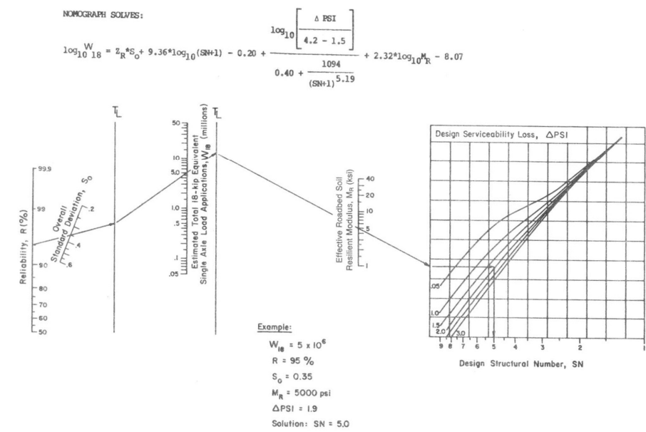
Design Chart for Flexible Pavements Based on Using Mean Values for Each Input
