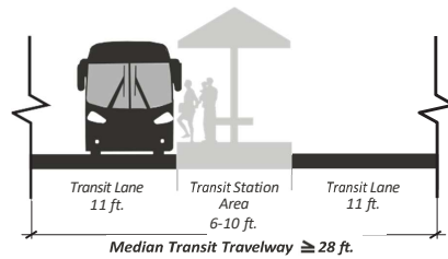
FIGURE 7.4.86 Median Transit Lanes and Center Platform Station
