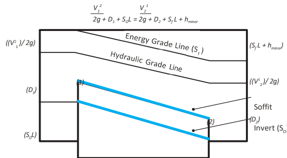
FIGURE 6.10.13 Hydraulic Grade
