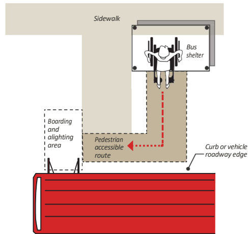
FIGURE 7.4.81 ADA/PROWAG-compliant Pedestrian Access Route
