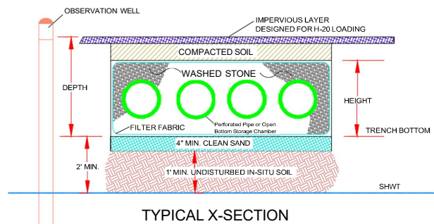
FIGURE 6.12.36 Infiltration Trench with Aggregate and Pipe Under Parking Lot
