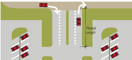
FIGURE 7.4.120 Throat Length
