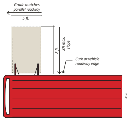
FIGURE 7.4.80 Transit Boarding and Alighting
