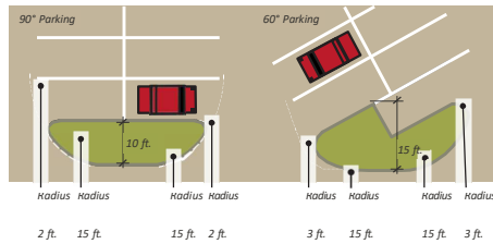
FIGURE 7.4.122 Parking Islands
