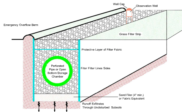
FIGURE 6.12.35 Infiltration Trench with Aggregate and Pipe
