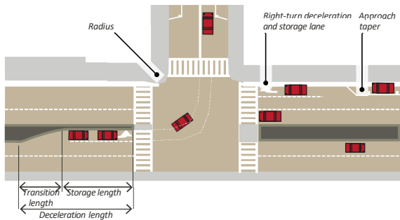
FIGURE 7.4.99 Turn Lane Design Elements
