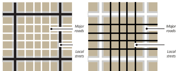
FIGURE 7.4.46 Regional and Neighborhood Roadway Networks
