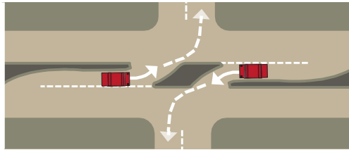
FIGURE 7.4.107 Restricted Median: Left-in Both Sides
