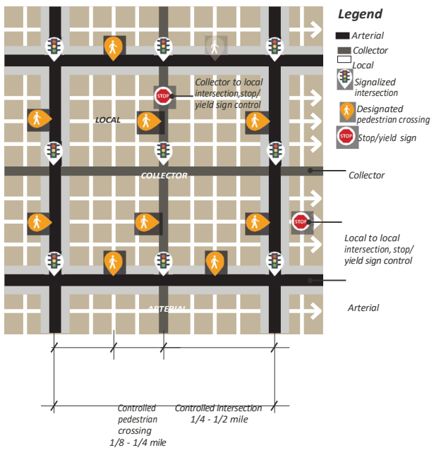
FIGURE 7.4.50 Example Layout: Signalized Intersections & Pedestrian Crossings
