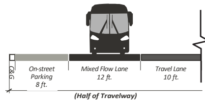
FIGURE 7.4.83 Travel Lane
