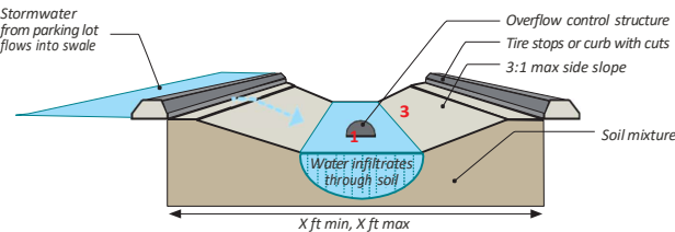
FIGURE 6.12.33 Landscape Conveyance-Bioswale
