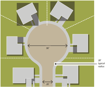
FIGURE 7.4.113 Cul-de-sac Dimensions
