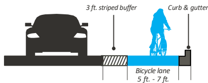
FIGURE 7.4.75 Bicycle Lane
