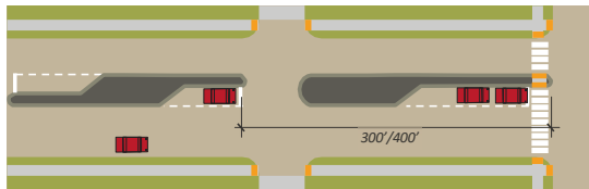
FIGURE 7.4.98 Median Opening Spacing
