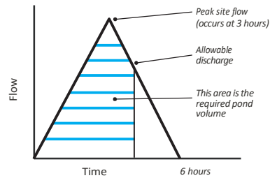
FIGURE 6.11.29 Peak Site Flow
