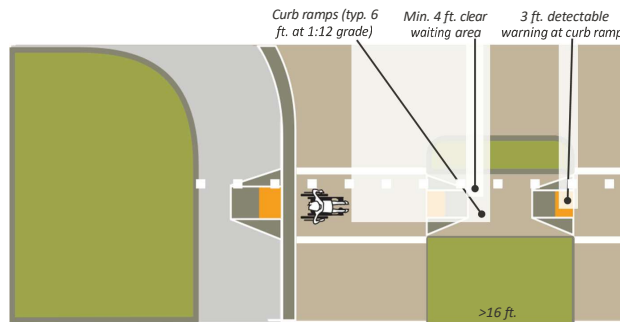
FIGURE 7.4.74 Refuge Island – Raised Median
