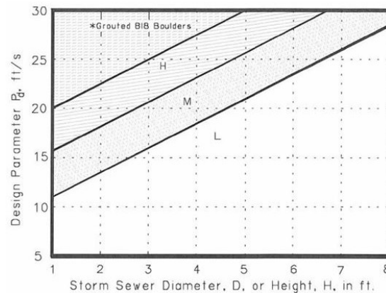
FIGURE 6.10.27 Low Trailwater Rip-rap Basins for Storm Sewer Pipe Outlets - Rip-rap Selection Chart for Low Tailwater Basin at Pipe Outlet
