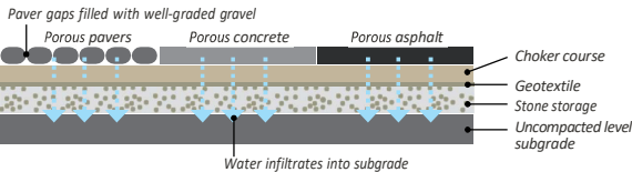
FIGURE 6.12.37 Porous Pavement with Typical Features
