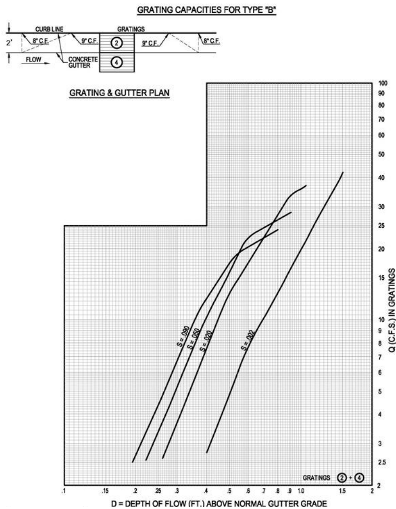
FIGURE 6.9.11 Grating Capacities for Type "B"
