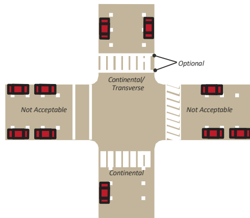
FIGURE 7.4.72 Crosswalk Marking
