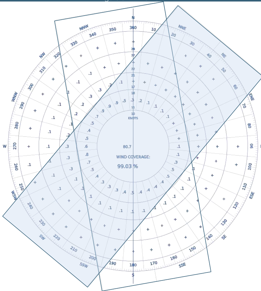
Figure 3.4 Wind Rose
