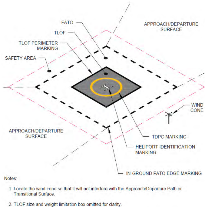
Figure 3.8 Basic Features of a General Aviation Heliport
