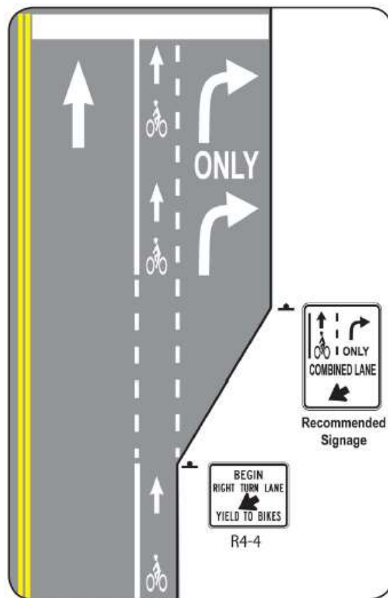
Recommended shared bike/right turn lane design.
