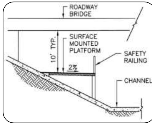
Figure 49: Trail Underpass Attached to Channel Surface
