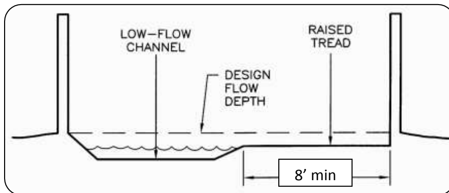
Figure 46: Neighborhood Trail Access via Shared Drainage Rundown
