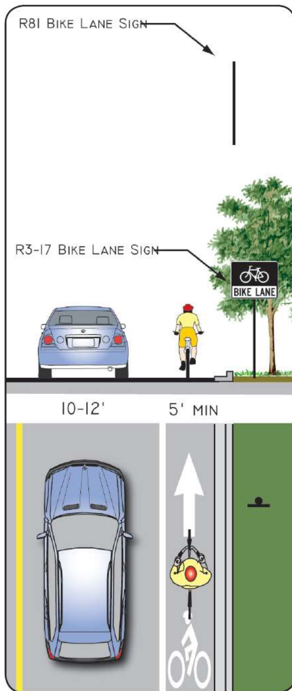
Recommend bike lane without on-street parking design.
