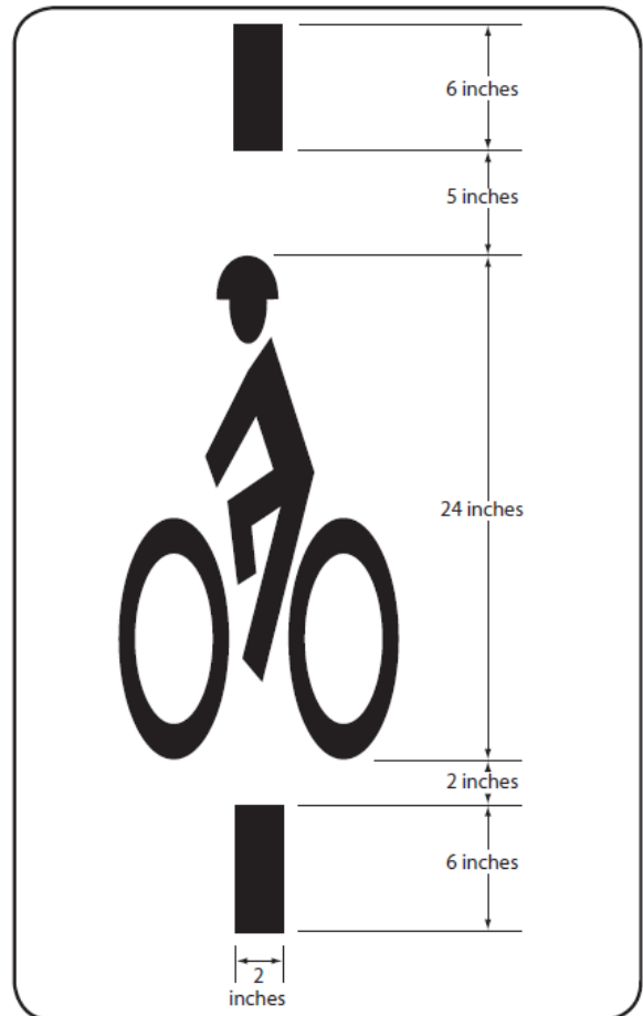
Recommended loop detector marking design.
