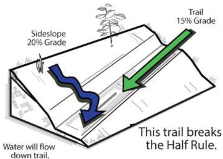
Figure 41: Sustainable Trail Design using the Half Rule Half Rule
