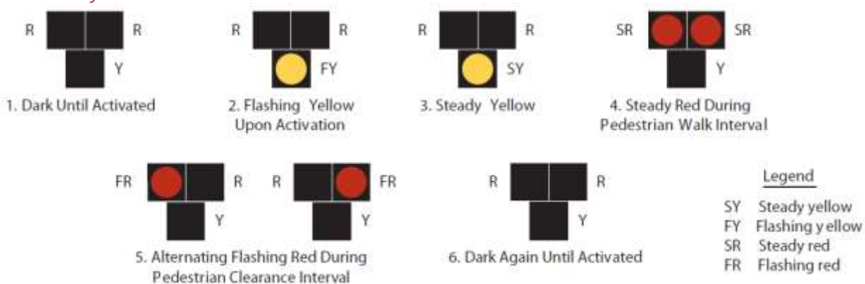
Sequence for a pedestrian hybrid beacon (MUTCD Figure 4F-3).
