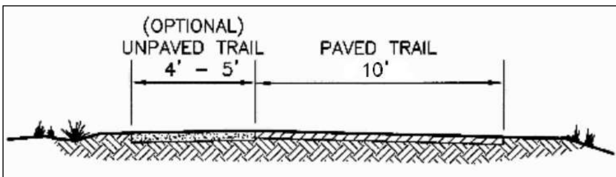
Figure 38: Typical Paved Multi-Use Trail Cross Section (no separation)
