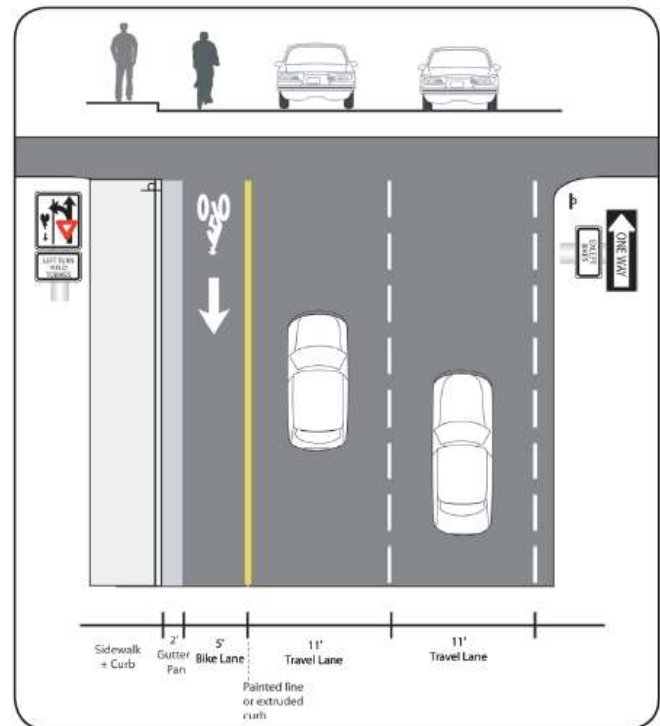
Recommended contraflow bike lane design.
