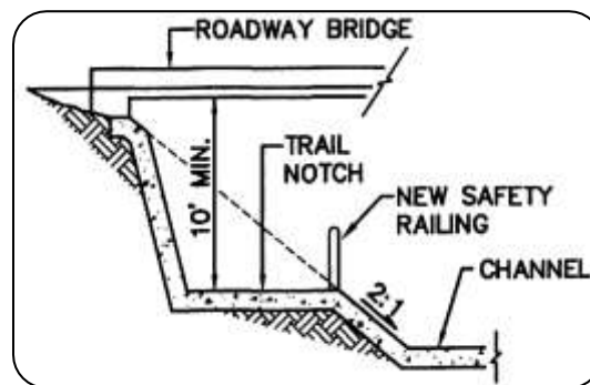
Figure 47: Trail Underpass Notched Into Side of Channel
