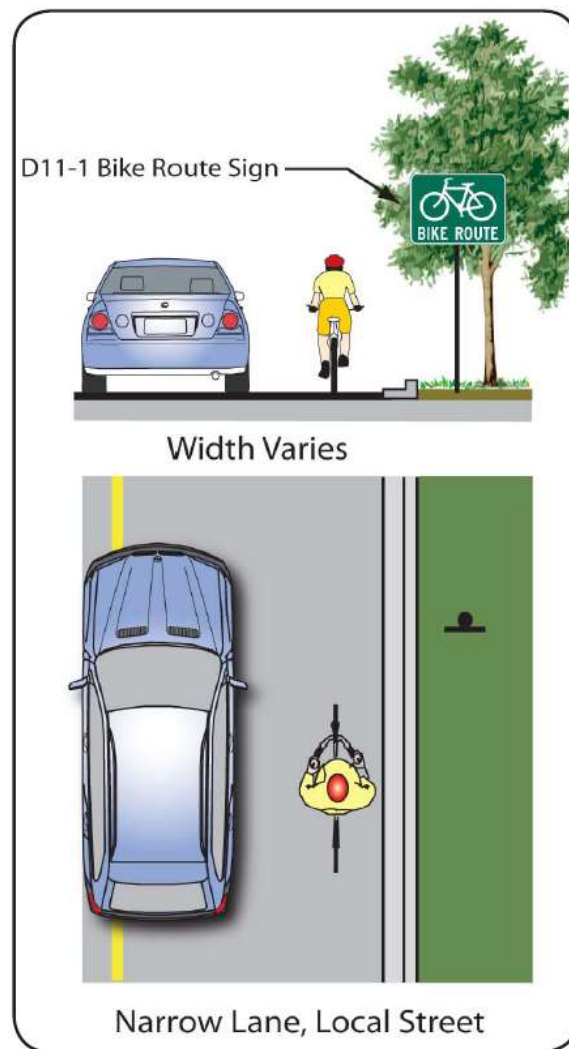
Recommended design for bike routes/ bicycle boulevards.
