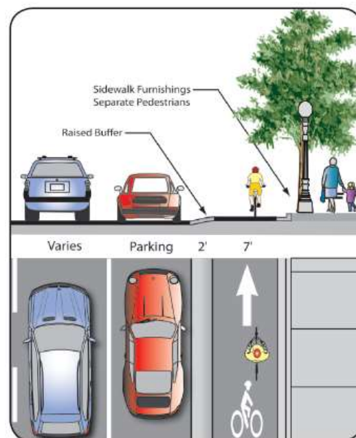
Recommended cycle track design with on-street parking.
