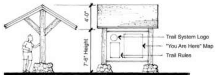
Figure 64: Trail Information Kiosk
