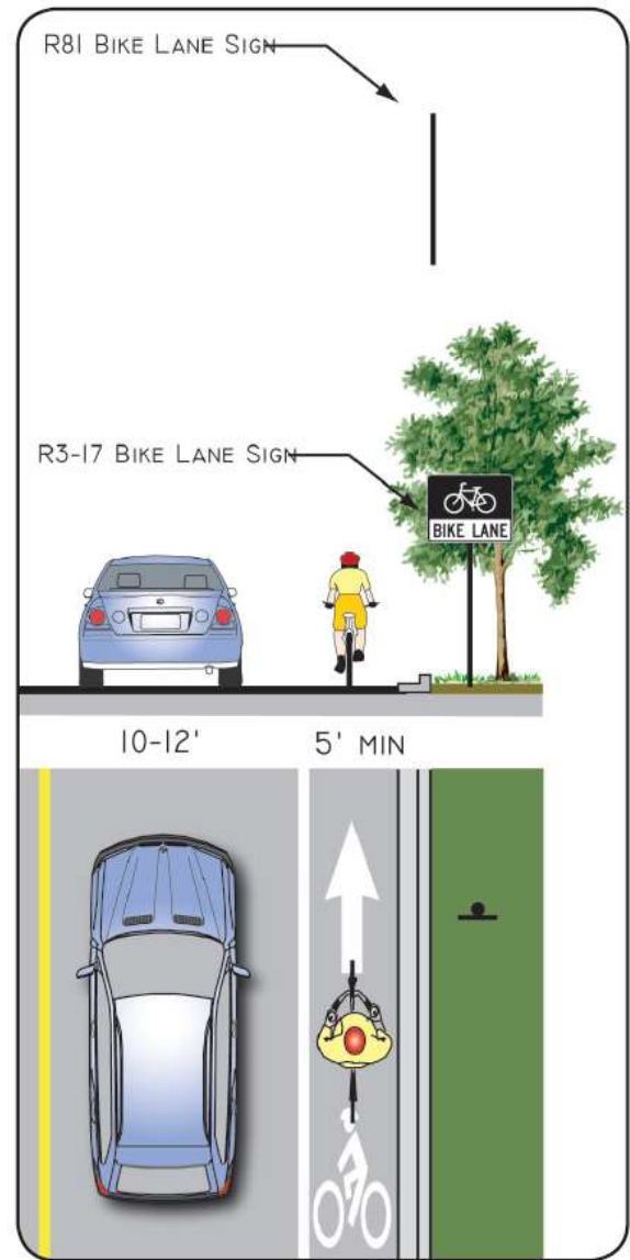
Recommended shoulder bikeway configuration.
