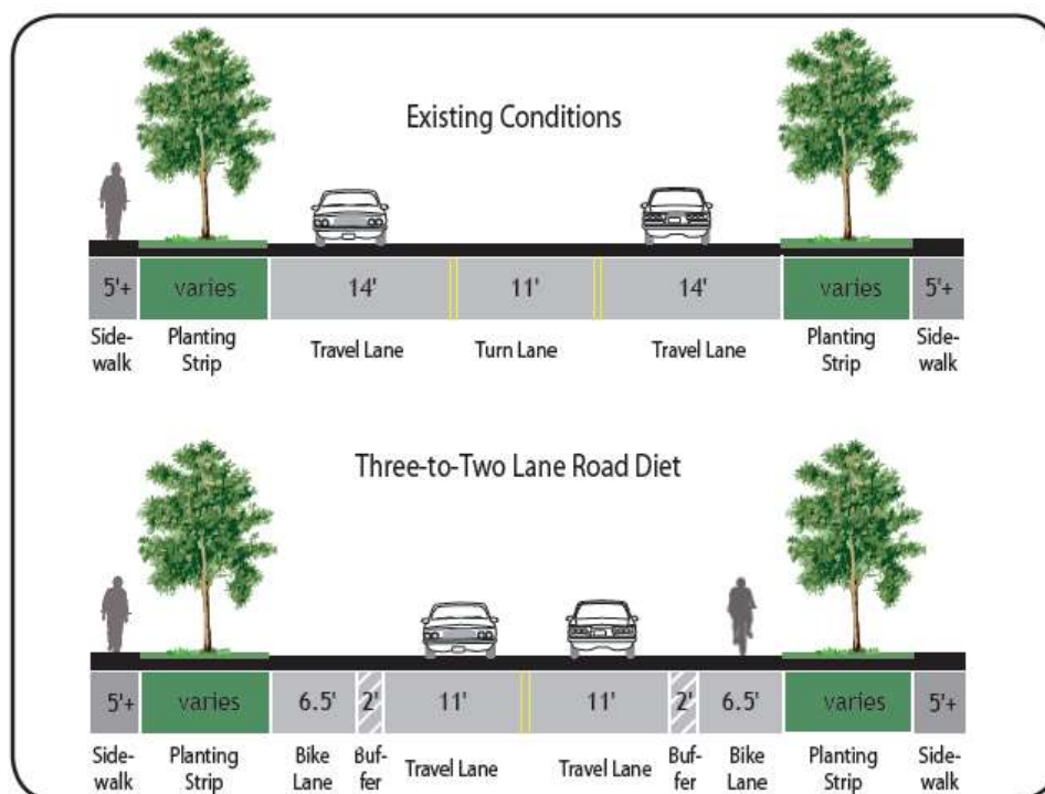
Example of vehicle travel lane reconfiguration to accommodate bike lanes.
