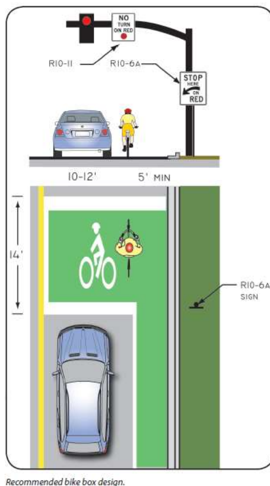
Recommended bike box design.
