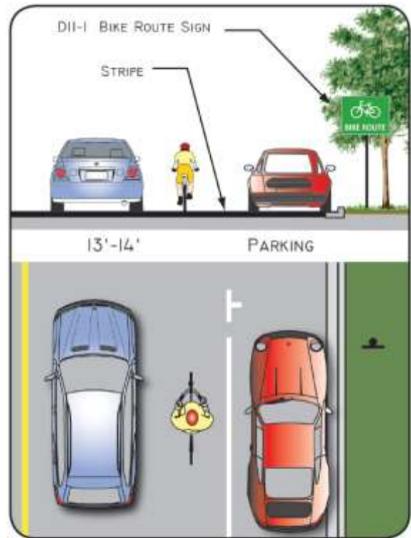
Shared roadway recommended configuration.
