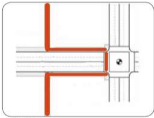
Type 2 Crossing Treatment.
