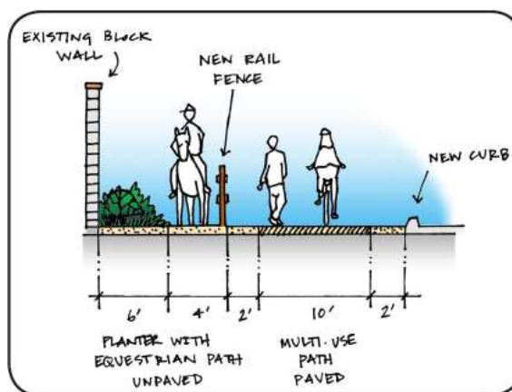
Recommended design for a multi-use path that accommodates equestrians.
