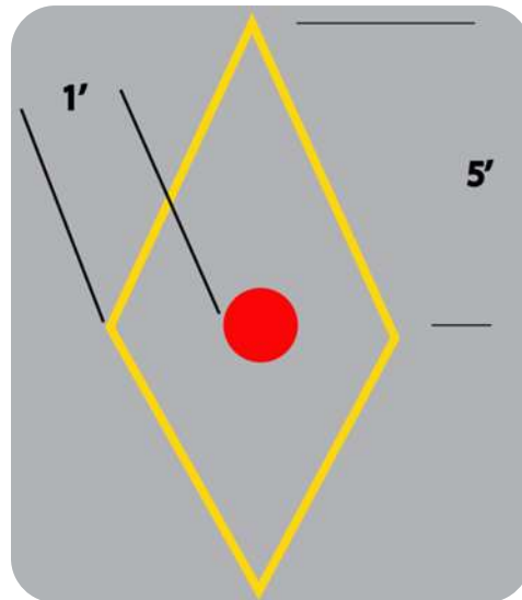
Figure 50: Typical Striping around Bollard
