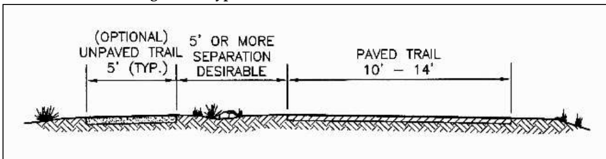
Figure 37: Typical Paved Multi-Use Trail Cross Section
