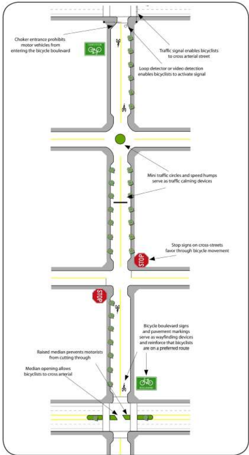
Sample bicycle boulevard treatments.
