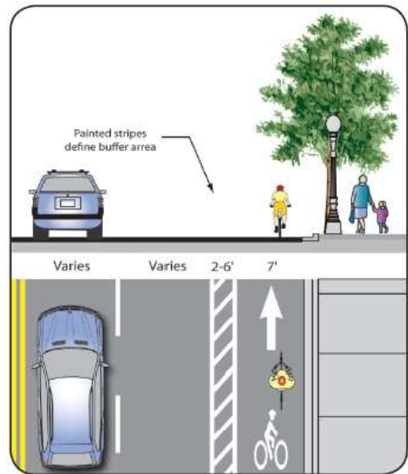
Recommended buffered bike lane design.
