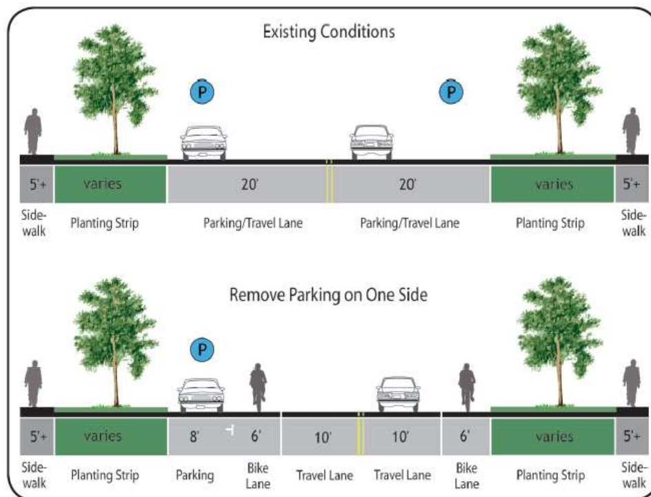
Example of parking removal to accommodate bike lanes.
