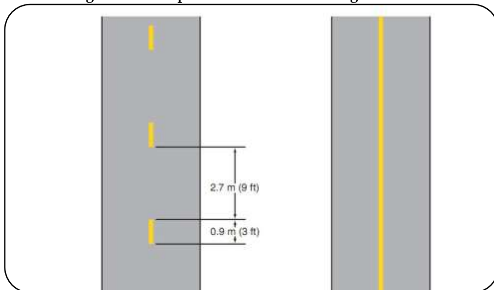
Figure 53: Examples of Centerline Markings for Trails
