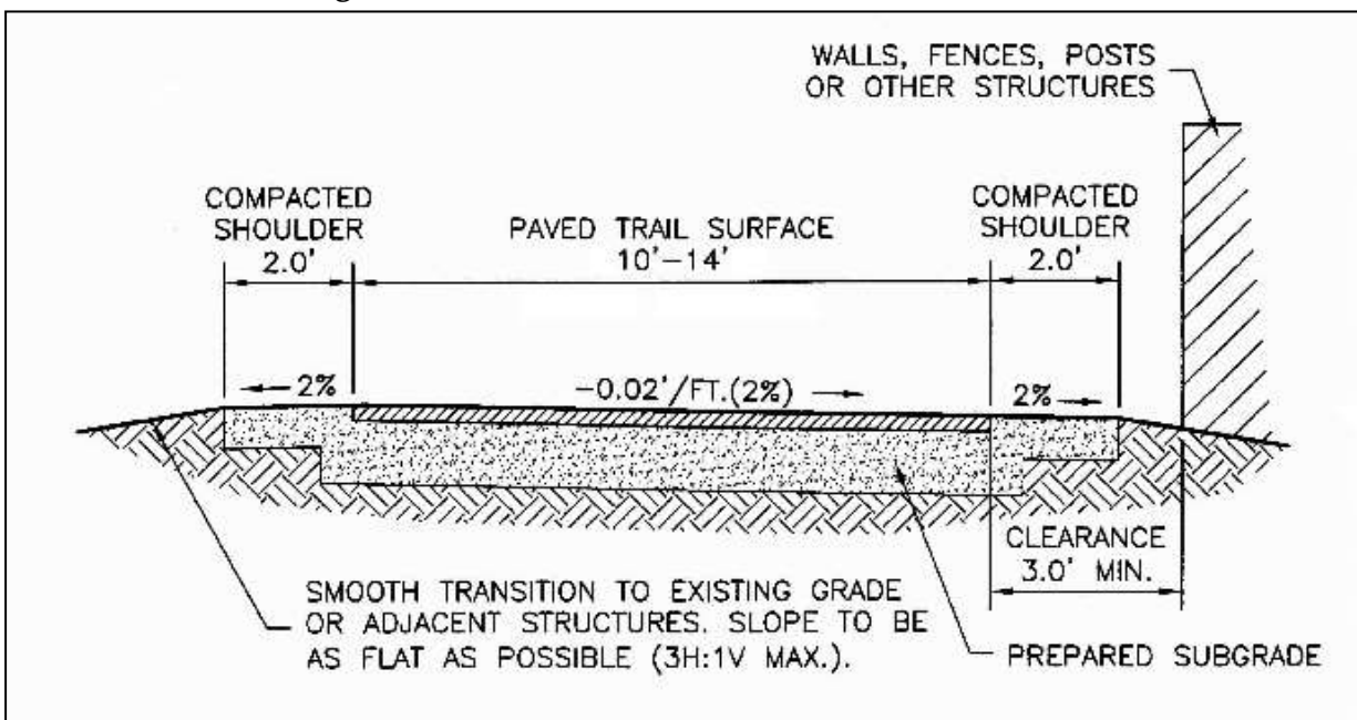
Figure 43: Paved Trail Dimensions and Clearances
