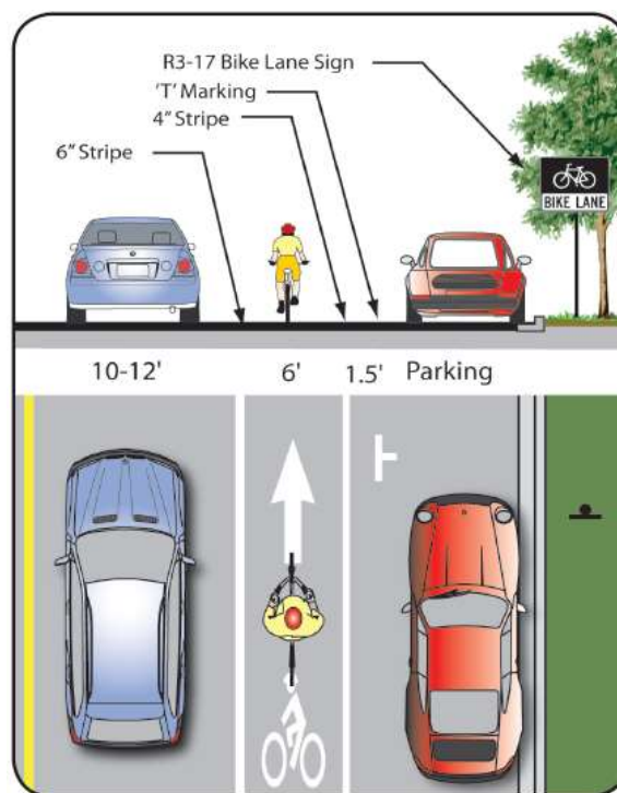
Parking buffer bike lane design.
