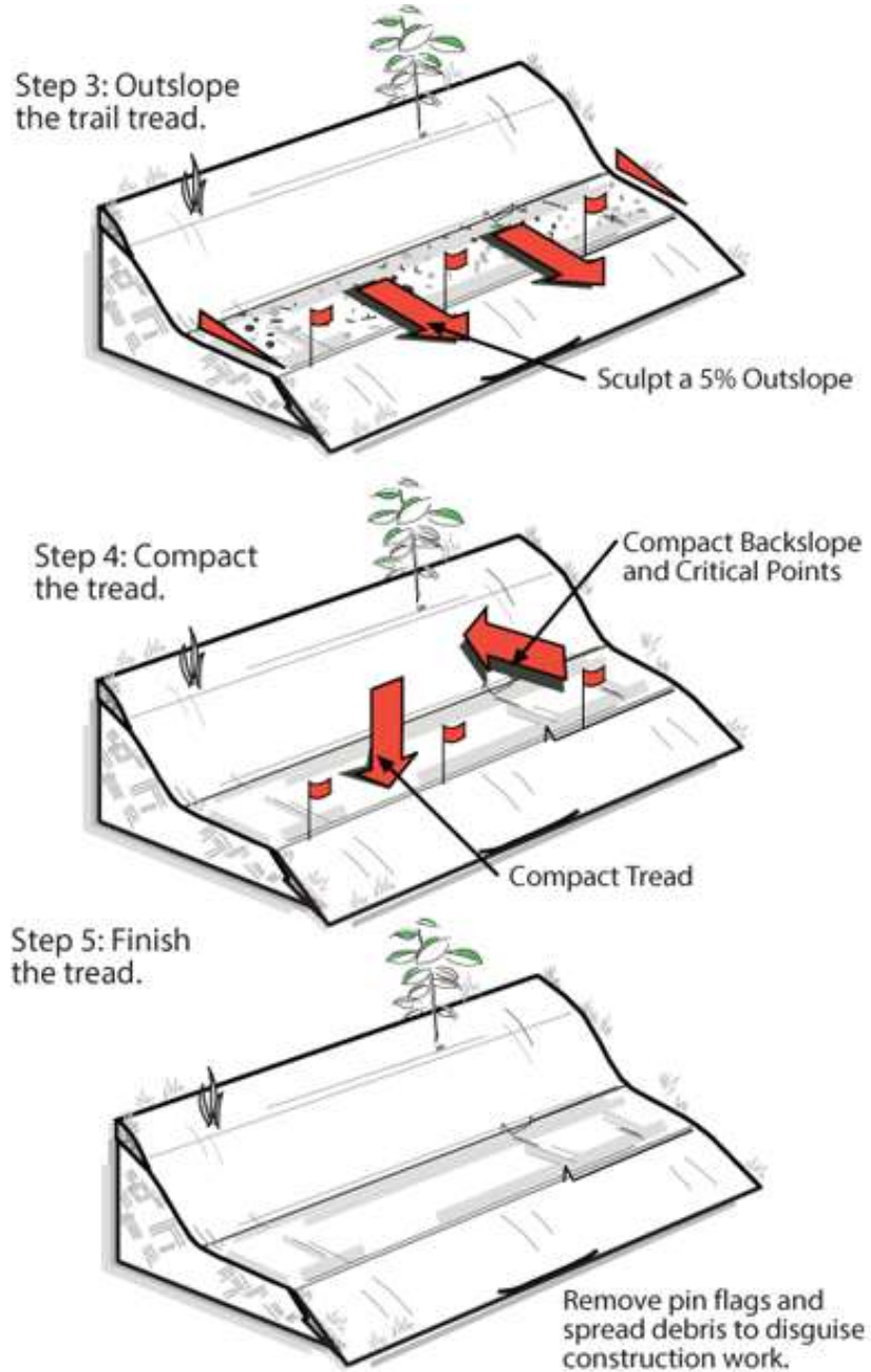
Figure 40: Typical MPOS Singletrack Full Bench Trail (cont.)
