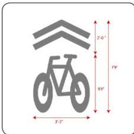
Figure 57: Sharrow Pavement Sign
