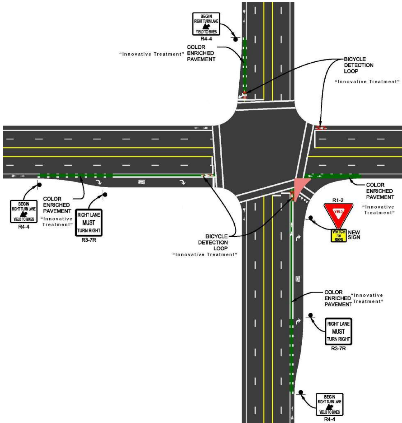
Figure 24: Prototypical Multi-lane Arterial Intersection Design
