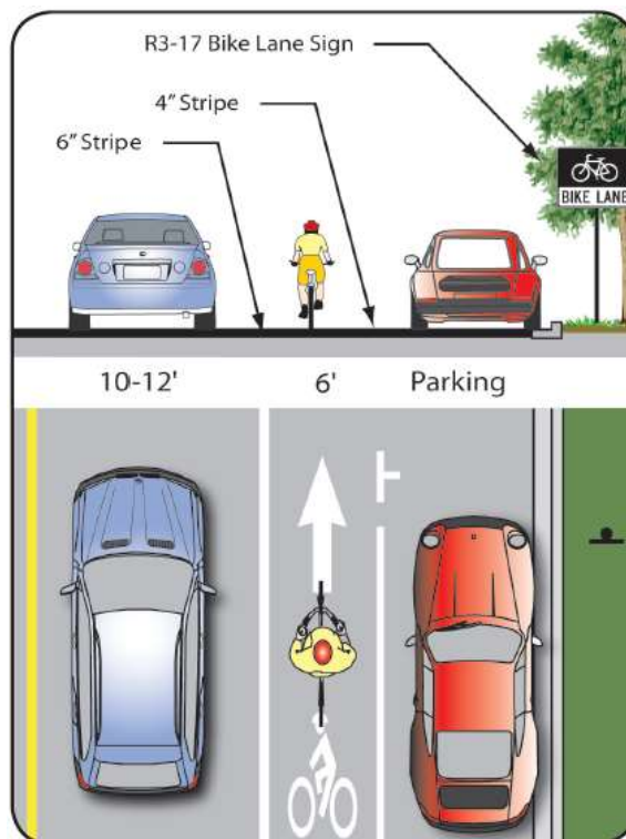
Parking 'T' bike lane design.
