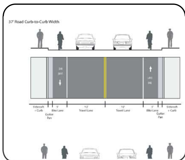
Two Lane Cross-Section with No Parking*. *Bike lanes may be 4' in width under constrained circumstances.
