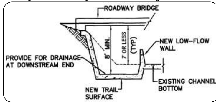
Figure 48: Depressed Underpass for Low Bridge Clearance Condition
