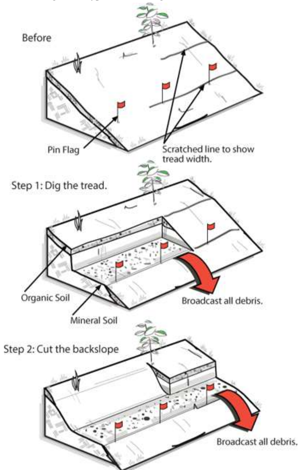
Figure 39: Typical MPOS Singletrack Full Bench Trail
