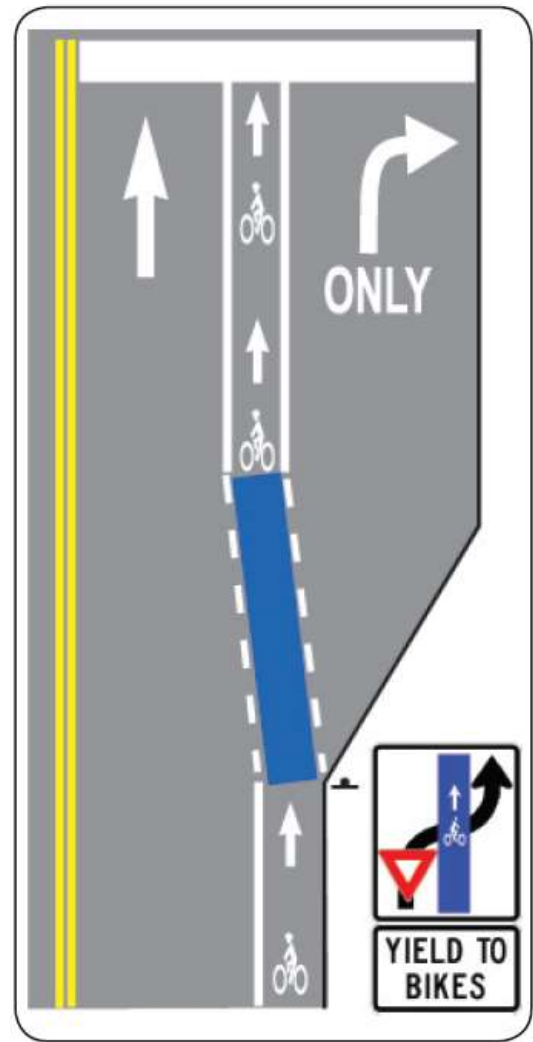
Recommended colored bike lane design.
