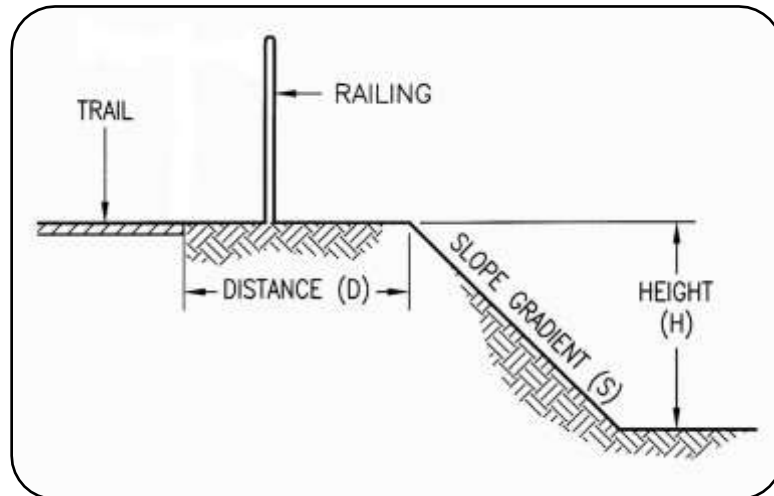
Figure 52: Railing Warrants
